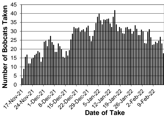
Figure 3. Estimated number of bobcats taken per day during the 2021-22 furharvesting season. (Data smoothed: y_{(i)} = .5y_{(i)} + .25y_{(i+1)} + .25y_{(i-1)} .)
